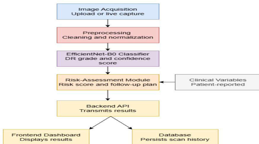
Fig1: System Workflow Diagram
