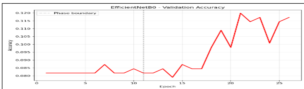
Fig. 3. Validation accuracy over epochs.
