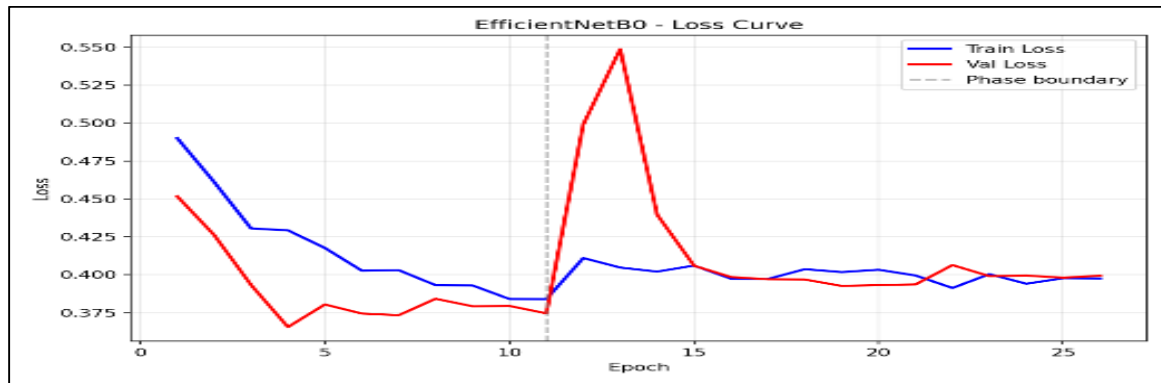
Fig. 4. Training and validation loss over epochs.
