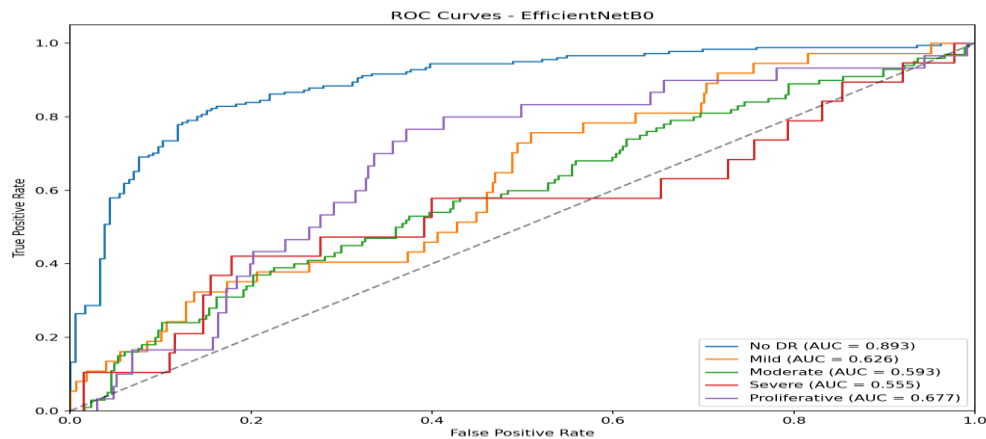
Fig. 5. One-vs-rest ROC curves per class.
