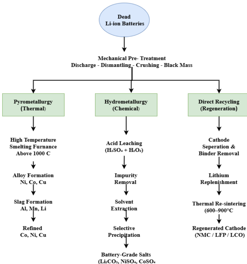
Figure 3: Flowchart of the recycling methods [30]
