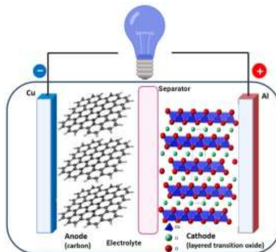
Figure 1: Components of LIBs: cathode, anode, electrolyte, and separator [10]
