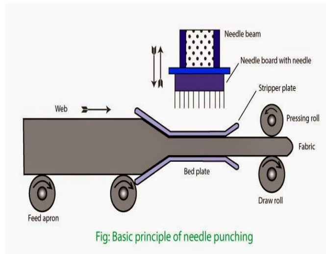
Figure 2 Needle punching technique
