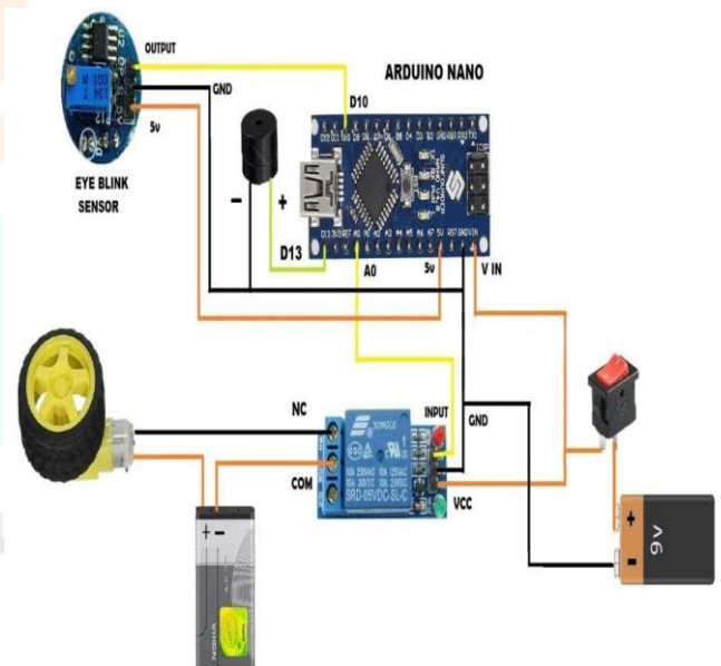
Figure 8: Final Connection of the Block
