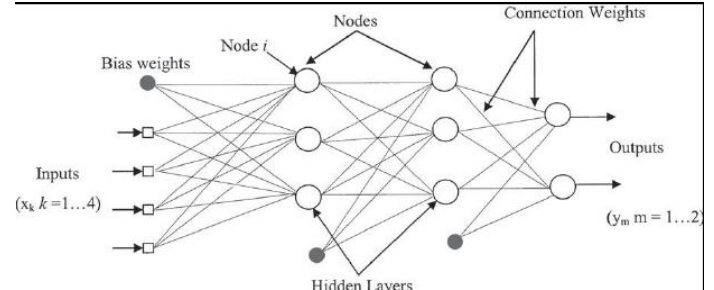
Figure 4: feedforward multi-layer network
