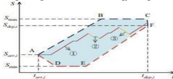
Fig. 2 Single Electric Vehicle energy storage model
