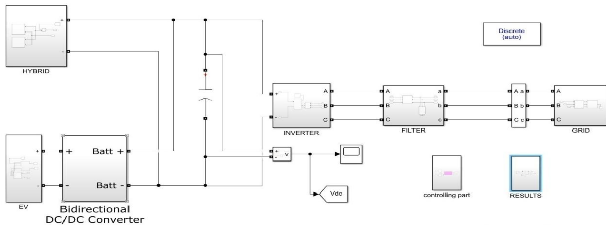
Fig. 9 Block Diagram of Hybrid integrated electric vehicle to grid
