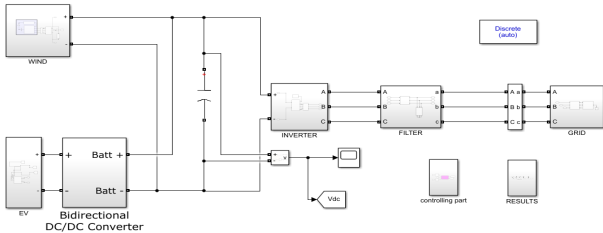
Fig. 5 Block Diagram of wind integrated electric vehicle to grid
