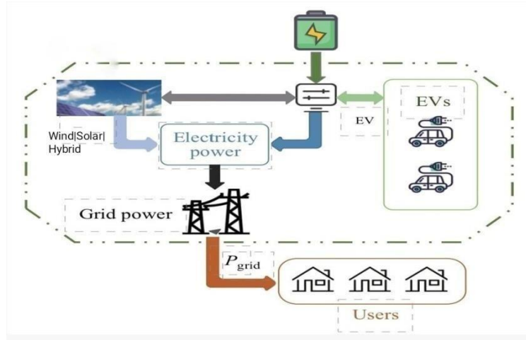
Fig. 1 Hybrid Energy Storage System Architecture
