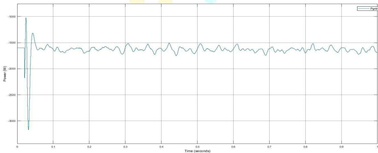
Fig. 6 Grid output power waveform with EV at wind power integration.
