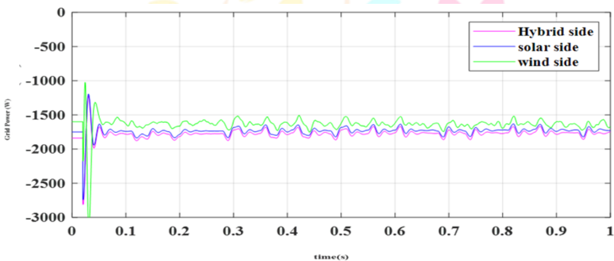
Fig. 11 Grid output power waveform with EV at wind, solar, hybrid power integration.
