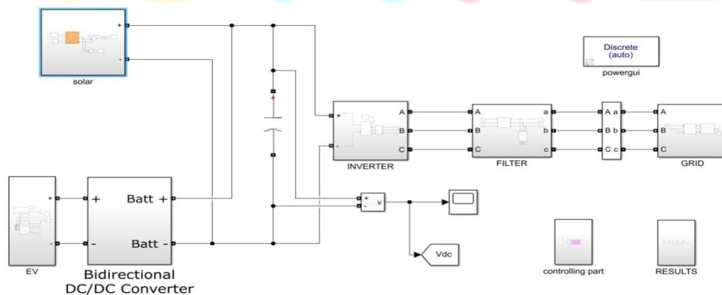
Fig. 7 Block Diagram of solar integrated electric vehicle to grid
