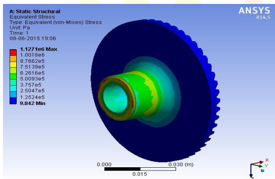
Fig.6 Static structural Equivalent stress
