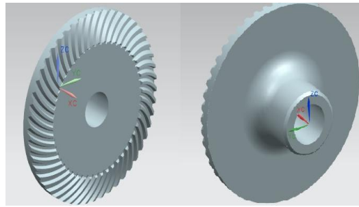
Fig.1 3D model of plain spiral bevel gear
