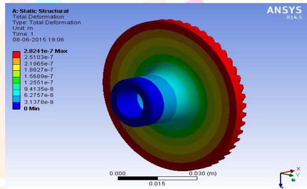
Fig.7 Static structural total deformation.
