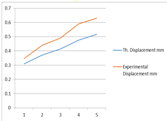
Graph 5. Load vs Displacement Graph
