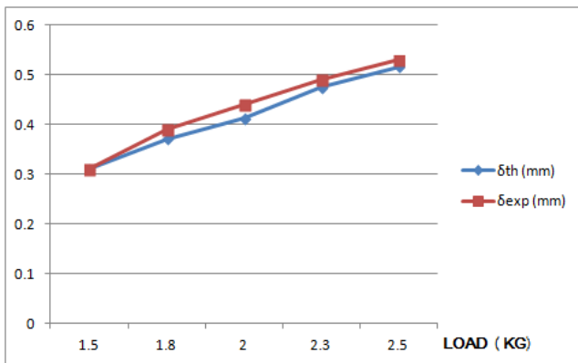
Graph 1. Load vs. Displacement
