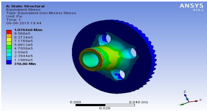
Fig.13 Static structural Equivalent stress.
