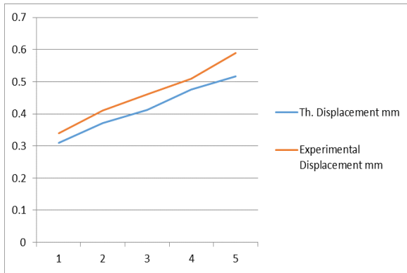
Graph 3 Load vs Displacement
