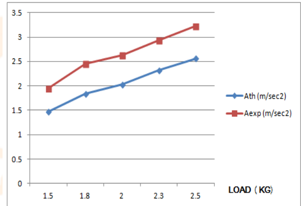
Graph 6 Load vs Acceleration
