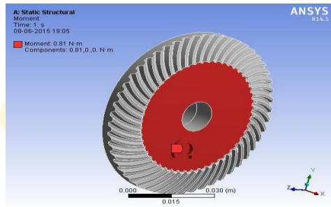
Fig.5 Applying Load
