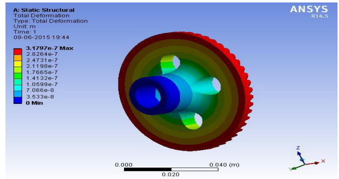
Fig.14 Static structural total deformation.
