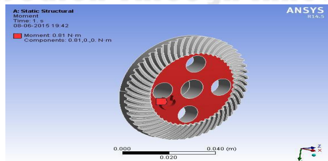
Fig.12 Applying Load
