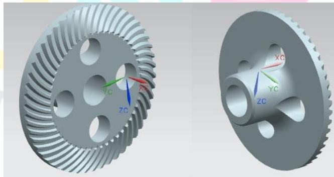
Fig 8 Spiral bevel gear: hole
