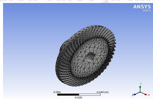
Fig.3 After Meshing
