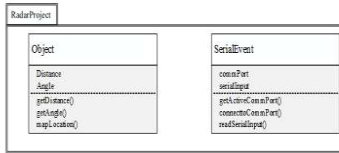
Figure 5. UML Class Diagram for GUI sub-system.
