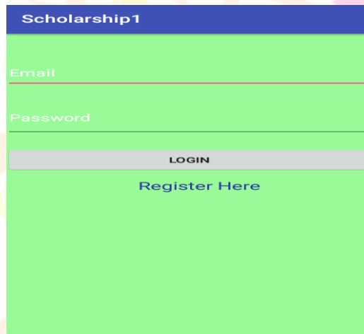
Figure 5: Login Page
