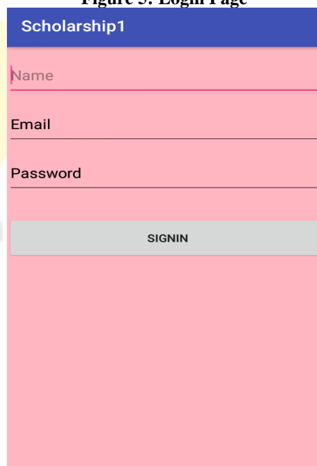
Figure 6: Login page
